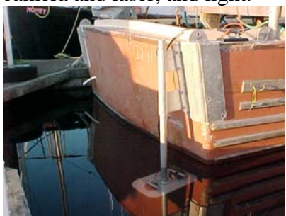
Echosounder transducers.
