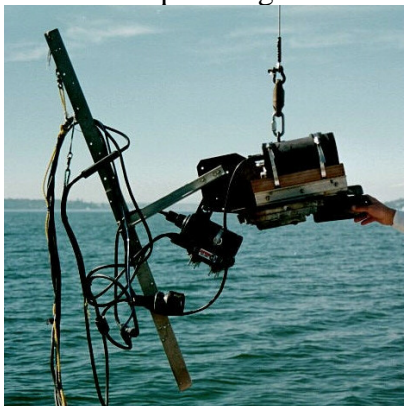
Towfish with HydroScat-2 (near hand), camera and laser, and light.
