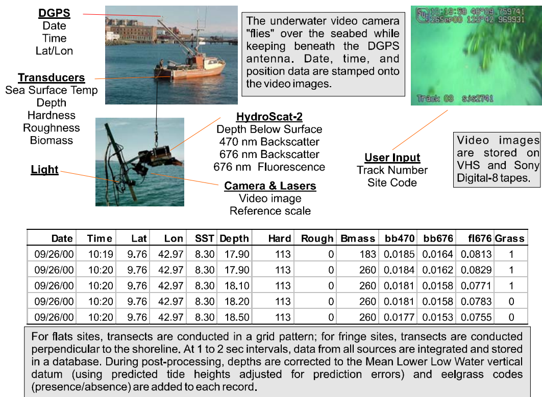
Figure 4. Illustration of the underwater videographic survey system.
