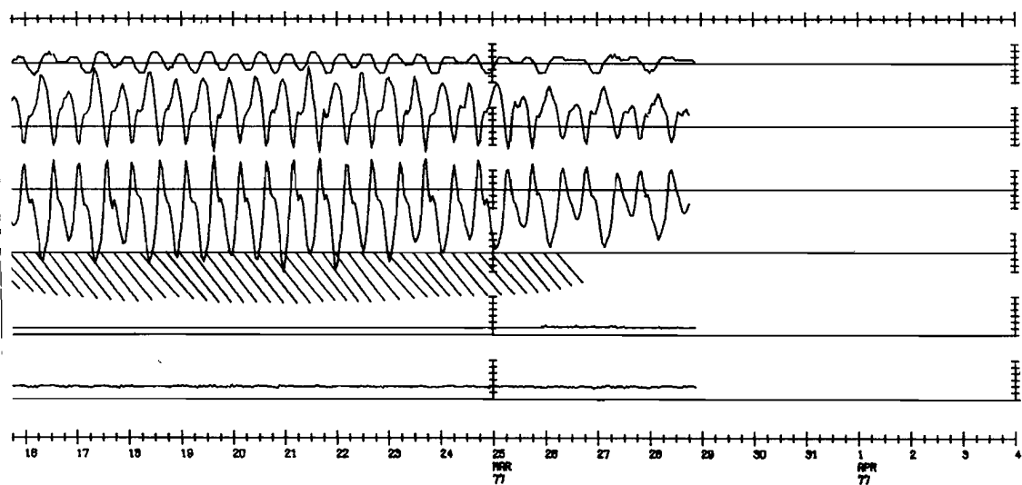
Figure 13. Pressure changes (m), currents (cm/sec), temperature ( ^{\circ}\text{C} ), and salinity ( ^{\circ}/\text{oo} ) for the near bottom meter at mooring 2 in The Narrows.
