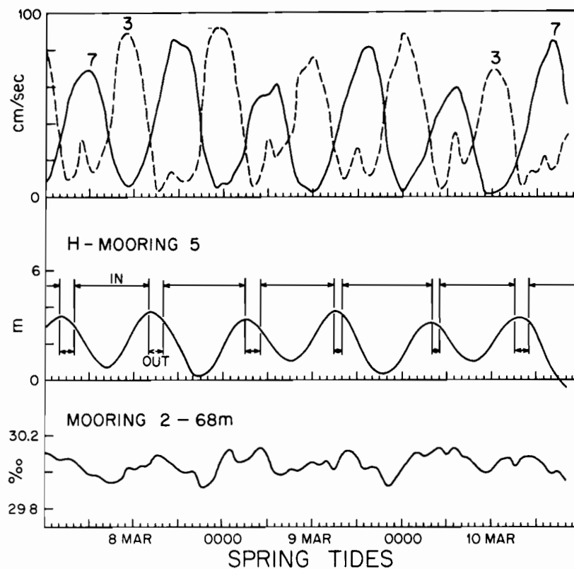
Figure 16. For neap and spring tides; hourly average speeds at moorings 3 and 7; tide height from mooring 5 indicating inflow (into The Narrows) or outflow at mooring 3; and salinity from near bottom at mooring 2.
