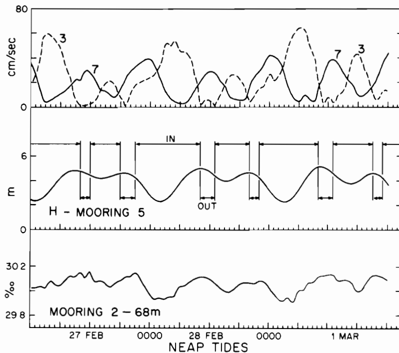
Figure 16. For neap and spring tides; hourly average speeds at moorings 3 and 7; tide height from mooring 5 indicating inflow (into The Narrows) or outflow at mooring 3; and salinity from near bottom at mooring 2.
